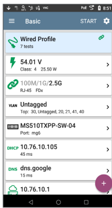
NBASE-T network with VLAN and 802.1x authentication
